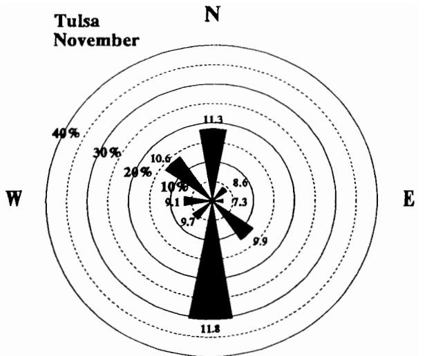
November Wind Roses for Oklahoma City and Tulsa. The frequency (percent) of winds from each direction is represented by length of its bar. The numbers at the ends of the bars indicate the average wind speed from that direction in miles per hour.
